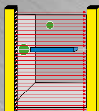
Figure 16/6 Ignore 1 beam only once
