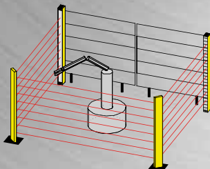
Light grid barriers for protection of access areas. Body protection.
