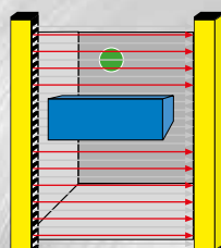
Figure 16/2 Fixed blanking with 1-beam reduced resolution
