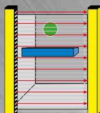
Figure 16/5 2-beam reduced resolution, any number of times
