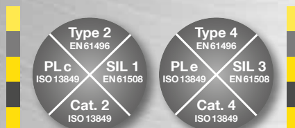
Light grid barriers for protection of access areas. Body protection.
