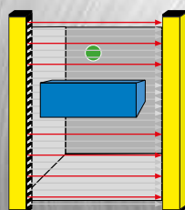
Figure 16/3 Fixed / floating blanking with 2-beam reduced resolution
