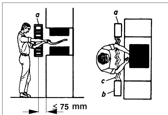
Fig. 15/1: Assembly without additional safeguarding
