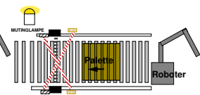
Cross-muting Differentiation between humans and material / machines
