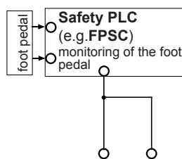
wiring diagram 4c/S.40 FUS FUO
