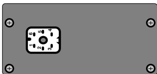
transmitter
