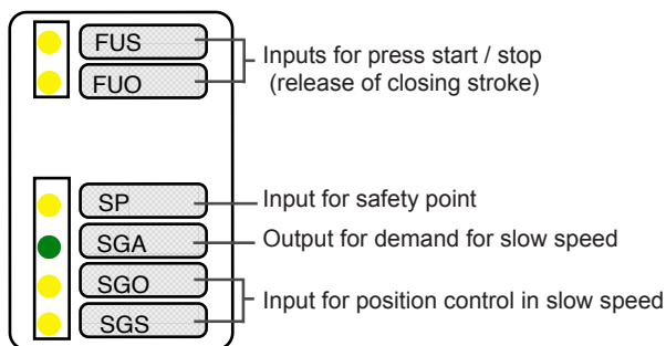
5 Indicator lights for in- and outputs (see page 47)
