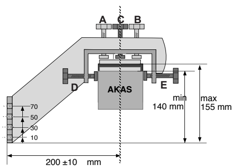
drawing, view from the top fig. 18/3
