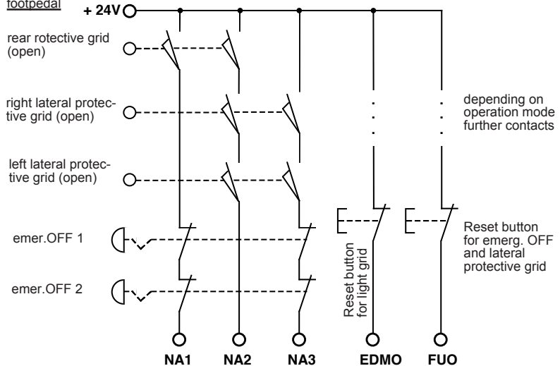
wiring diagram 5b/S.41
