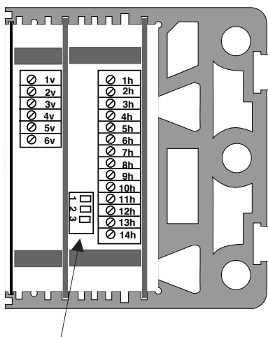
terminals receiver
